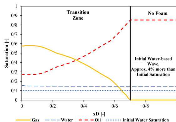
Fig. 4 Saturation profile in the matrix after one year. Mixed-wet matrix, with capillary pressure.
