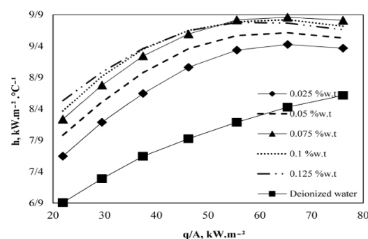
Fig. 3 Effect of CuO concentration on the BHTC relative to deionized water.
