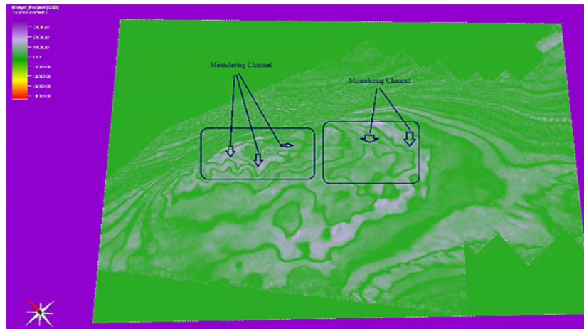
Fig. 1 Horizontal section of spectral decomposition attribute at a depth of (1960) m.
