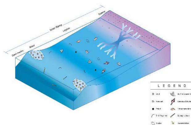
Fig. 2 Schematic block diagram of the Arab Formation in the studied field.
