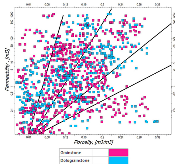
Fig. 5 Cross plot of porosity and permeability in grainstone and dolograstone facies.
