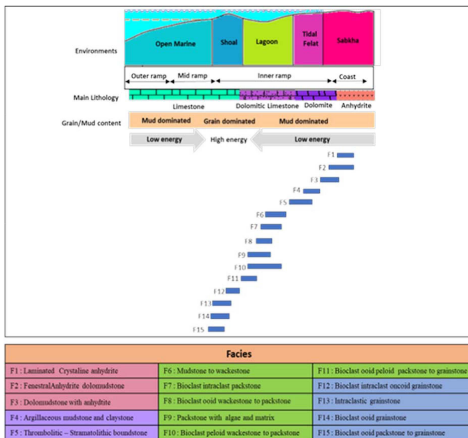
Fig. 2 Sedimentary environment model with microfacies.
