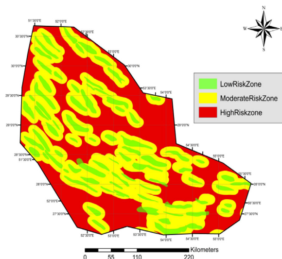
Fig.4 The final geological risk map.
