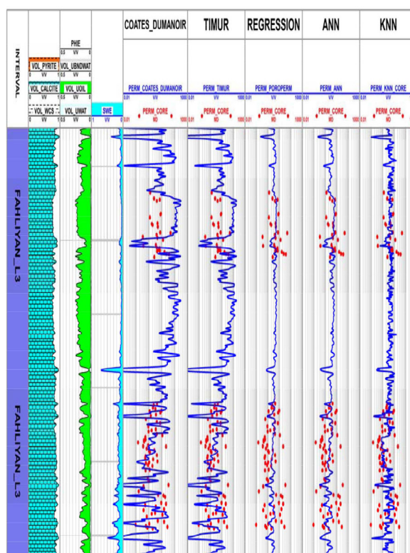
Fig. 1 Comparison of applying different methods for permeability prediction, Layer 3 of Fahlivan Formation, Well-C.
